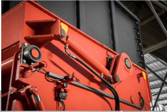
Hydraulically-moved swing ram with robust lever and swingarm bearing
