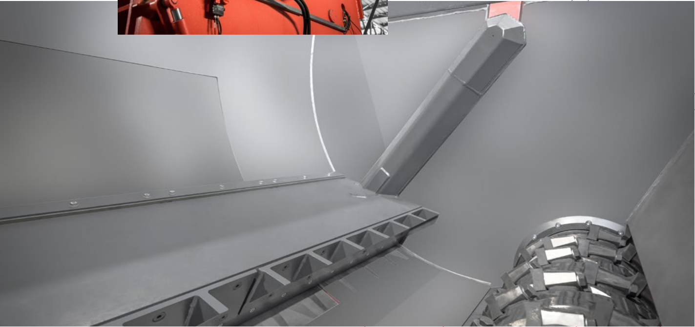
Hydraulically-moved swing ram with robust lever and swingarm bearing
